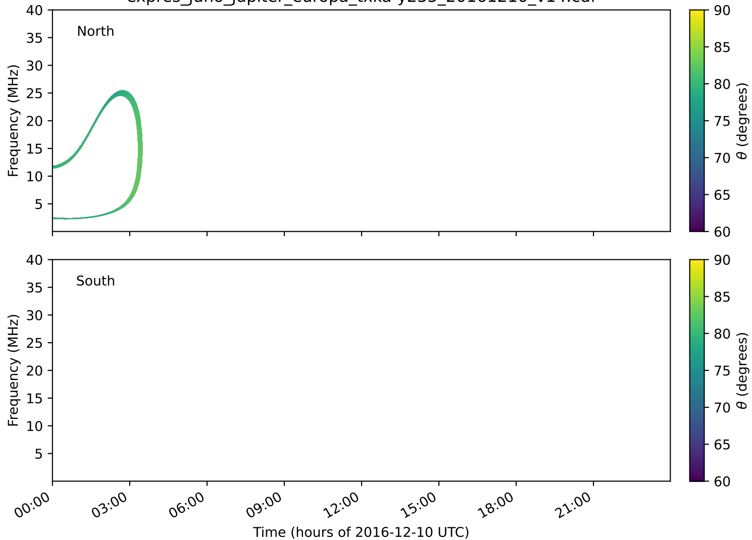
expres_juno_jupiter_europa_txka-y235_20161210_v14.cdf
