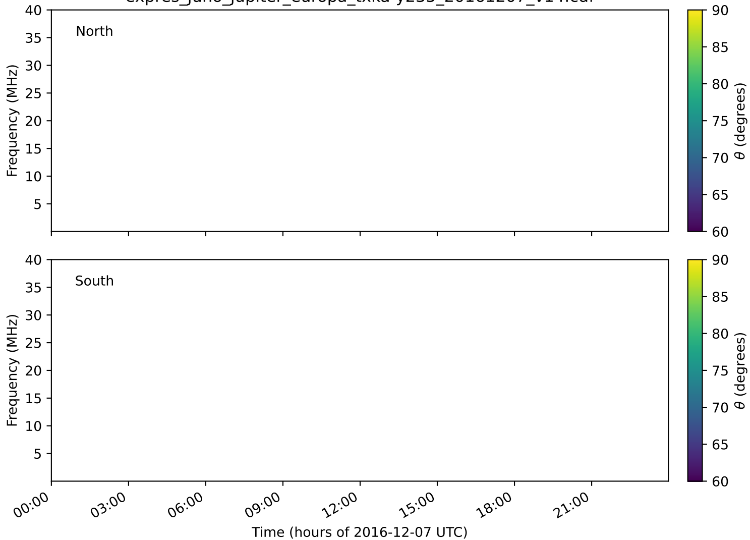
expres_juno_jupiter_europa_txka-y235_20161207_v14.cdf
