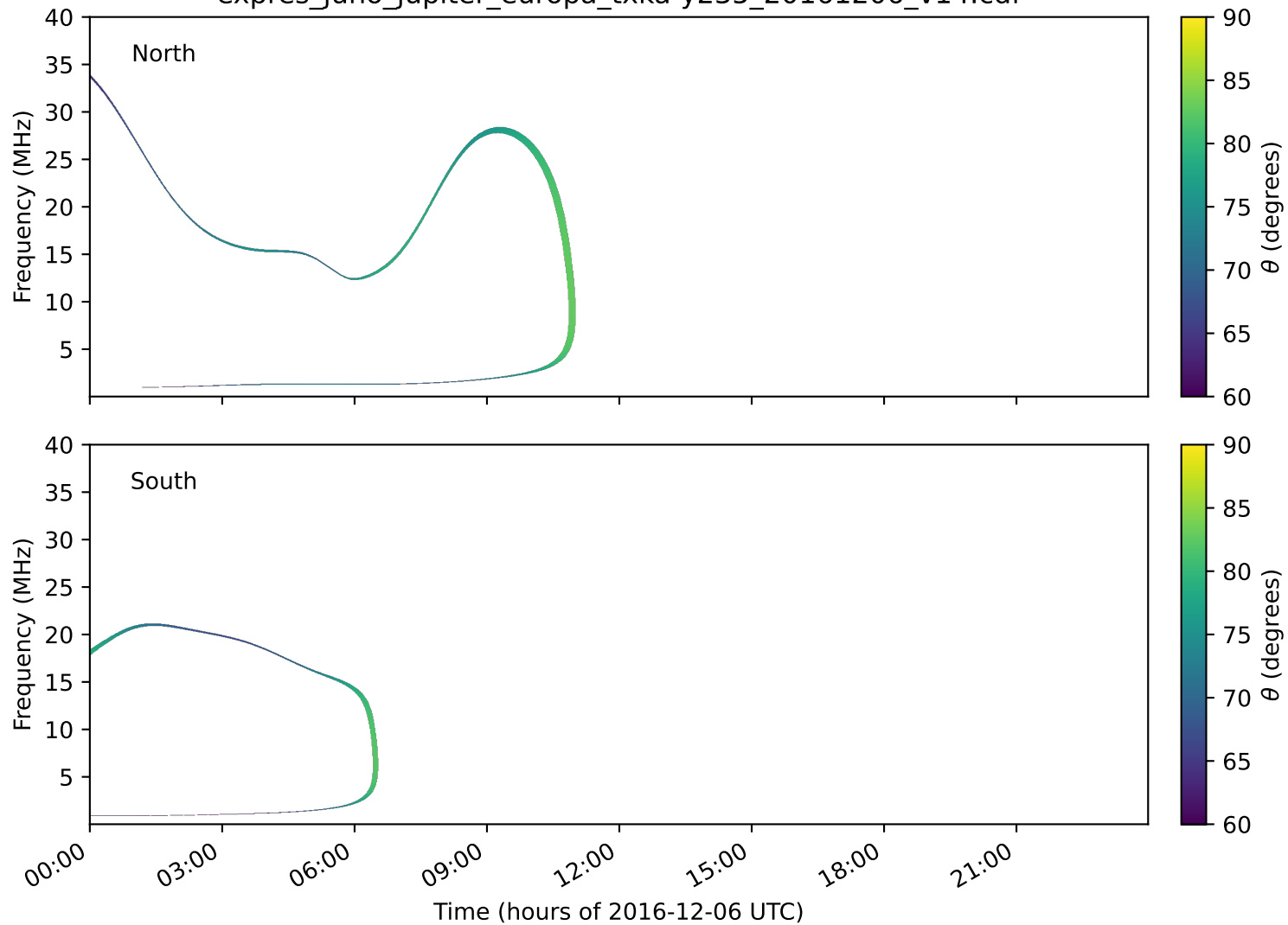
expres_juno_jupiter_europa_txka-y235_20161206_v14.cdf
