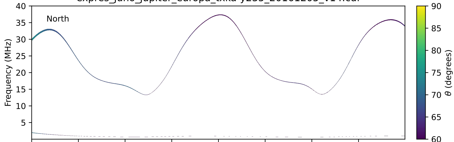
expres_juno_jupiter_europa_txka-y235_20161205_v14.cdf
