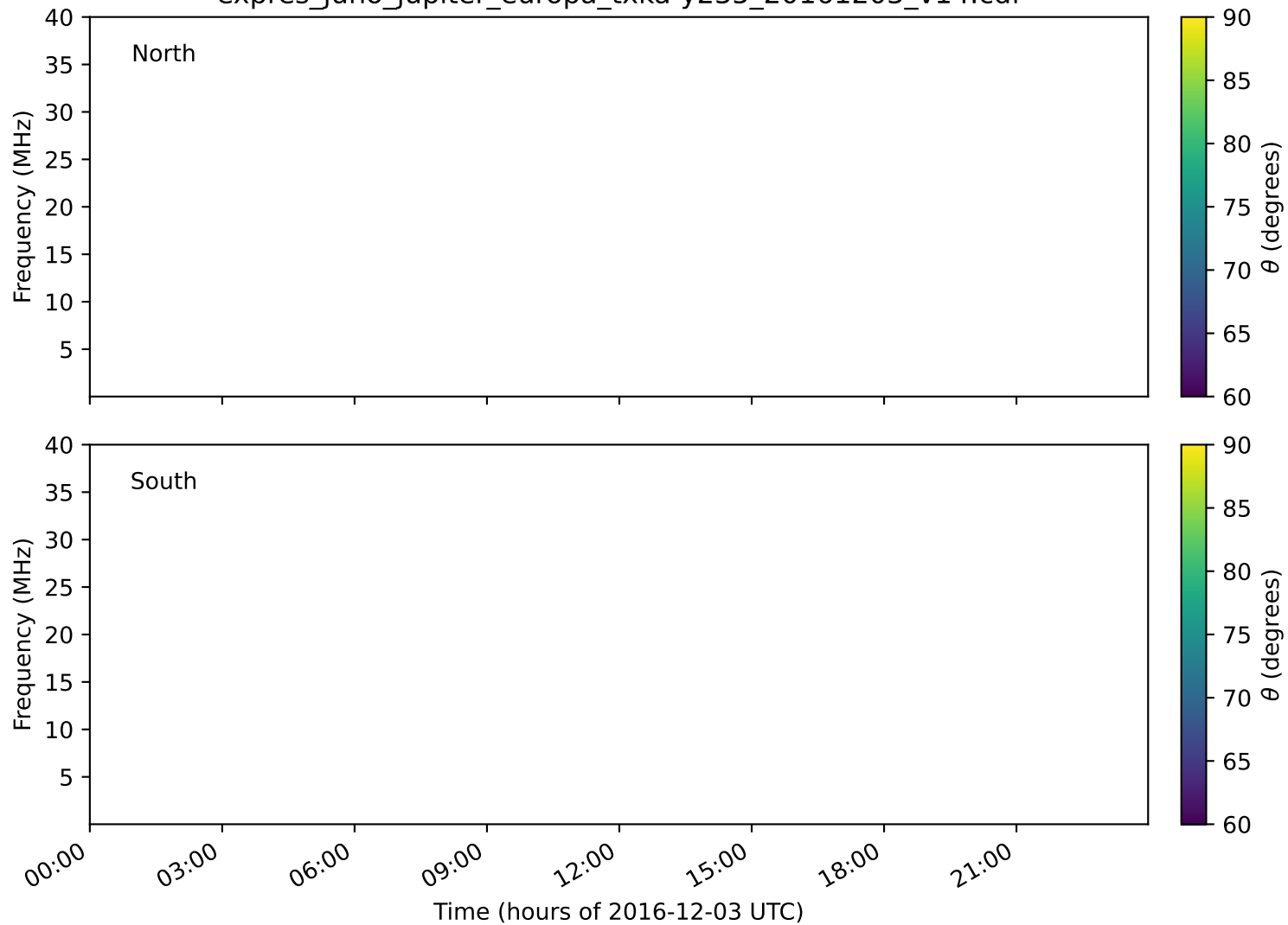
expres_juno_jupiter_europa_txka-y235_20161203_v14.cdf
