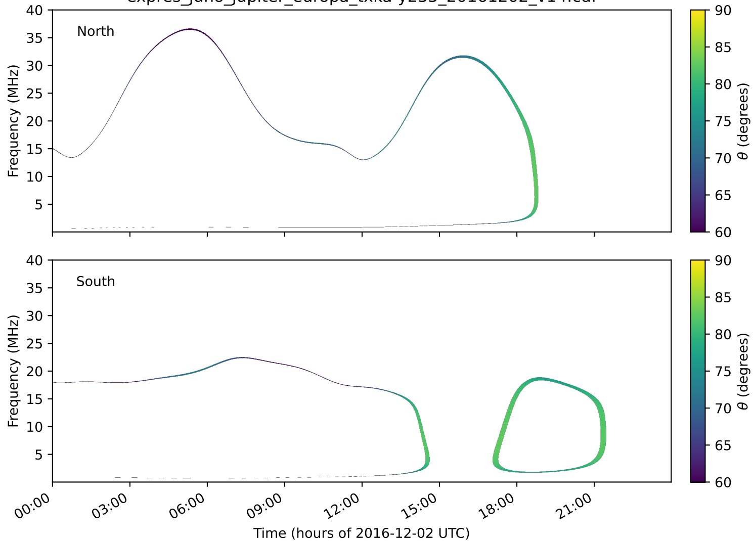
expres_juno_jupiter_europa_txka-y235_20161202_v14.cdf
