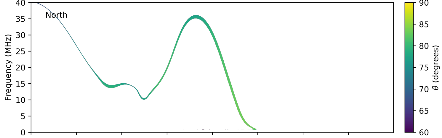
expres_juno_jupiter_europa_jrm09_lossc-wid1deg_3kev_20161227_v01.cdf
