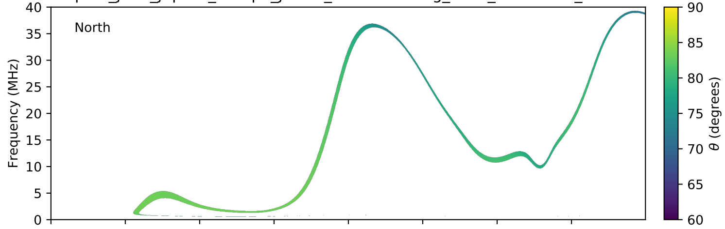
expres_juno_jupiter_europa_jrm09_lossc-wid1deg_3kev_20161219_v01.cdf
