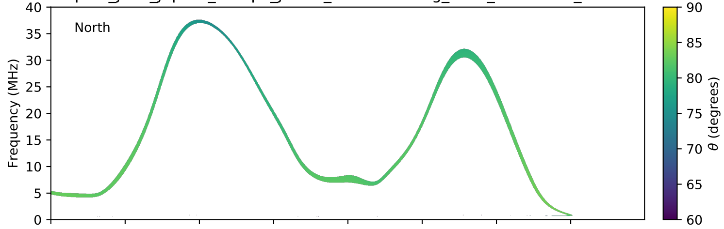
expres_juno_jupiter_europa_jrm09_lossc-wid1deg_3kev_20161216_v01.cdf
