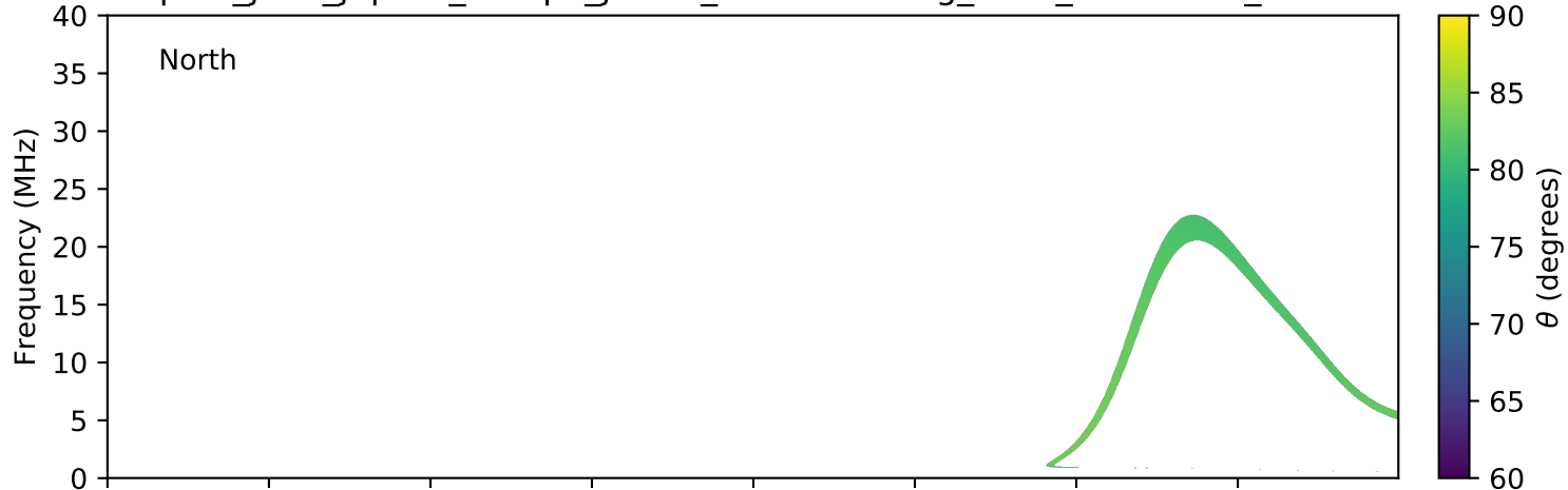
expres_juno_jupiter_europa_jrm09_lossc-wid1deg_3kev_20161215_v01.cdf
