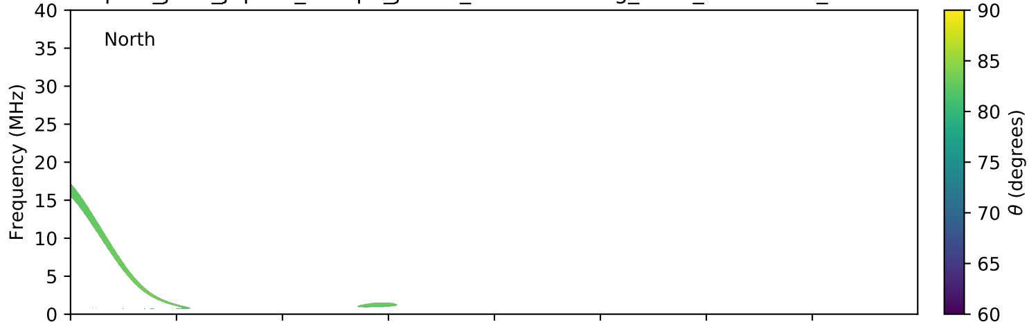
expres_juno_jupiter_europa_jrm09_lossc-wid1deg_3kev_20161213_v01.cdf
