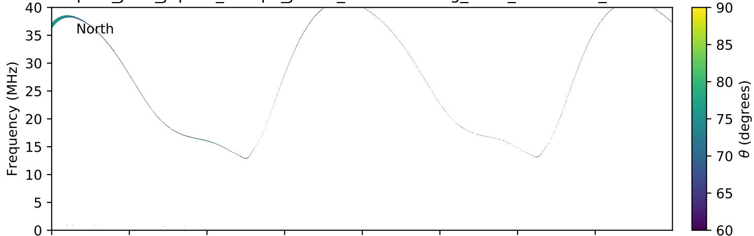
expres_juno_jupiter_europa_jrm09_lossc-wid1deg_3kev_20161205_v01.cdf
