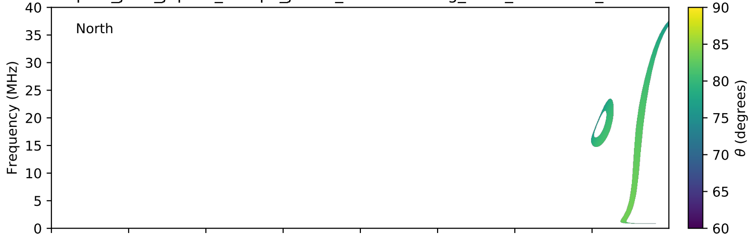
expres_juno_jupiter_europa_jrm09_lossc-wid1deg_3kev_20161204_v01.cdf
