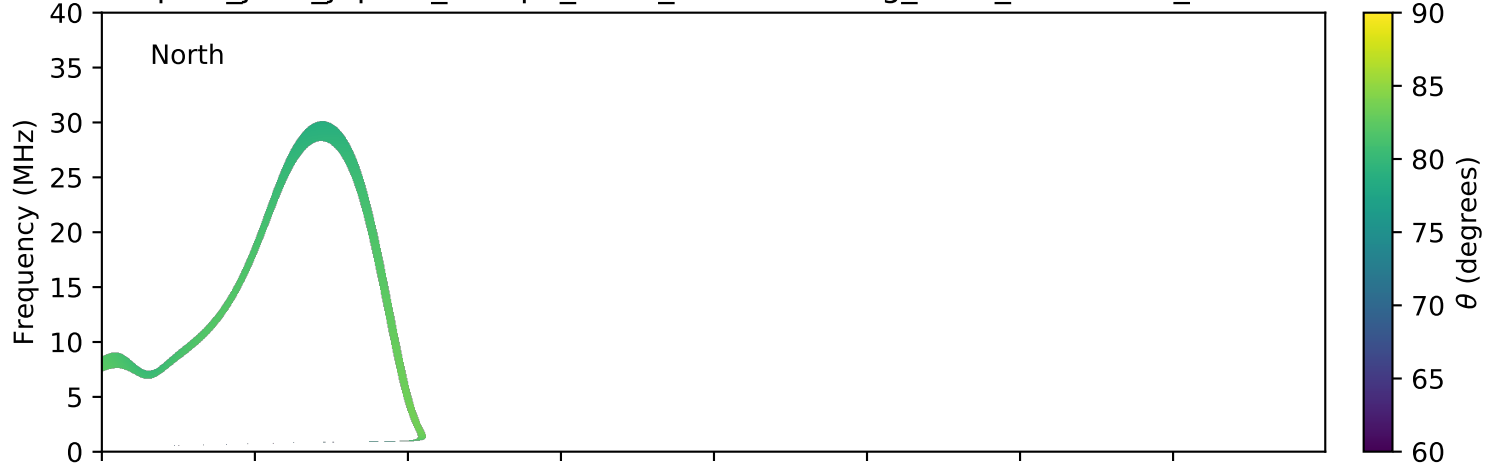
expres_juno_jupiter_europa_isaac_lossc-wid1deg_3kev_20161231_v01.cdf
