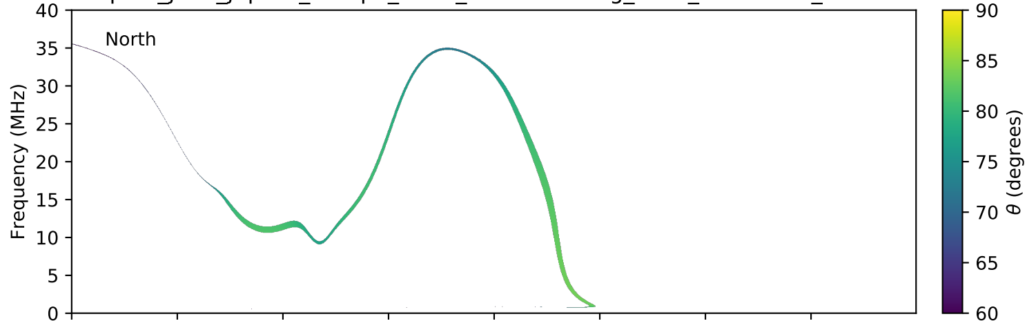
expres_juno_jupiter_europa_isaac_lossc-wid1deg_3kev_20161227_v01.cdf
