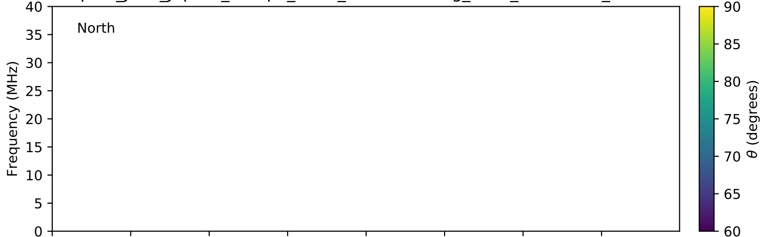
expres_juno_jupiter_europa_isaac_lossc-wid1deg_3kev_20161225_v01.cdf
