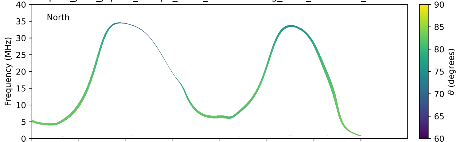
expres_juno_jupiter_europa_isaac_lossc-wid1deg_3kev_20161216_v01.cdf
