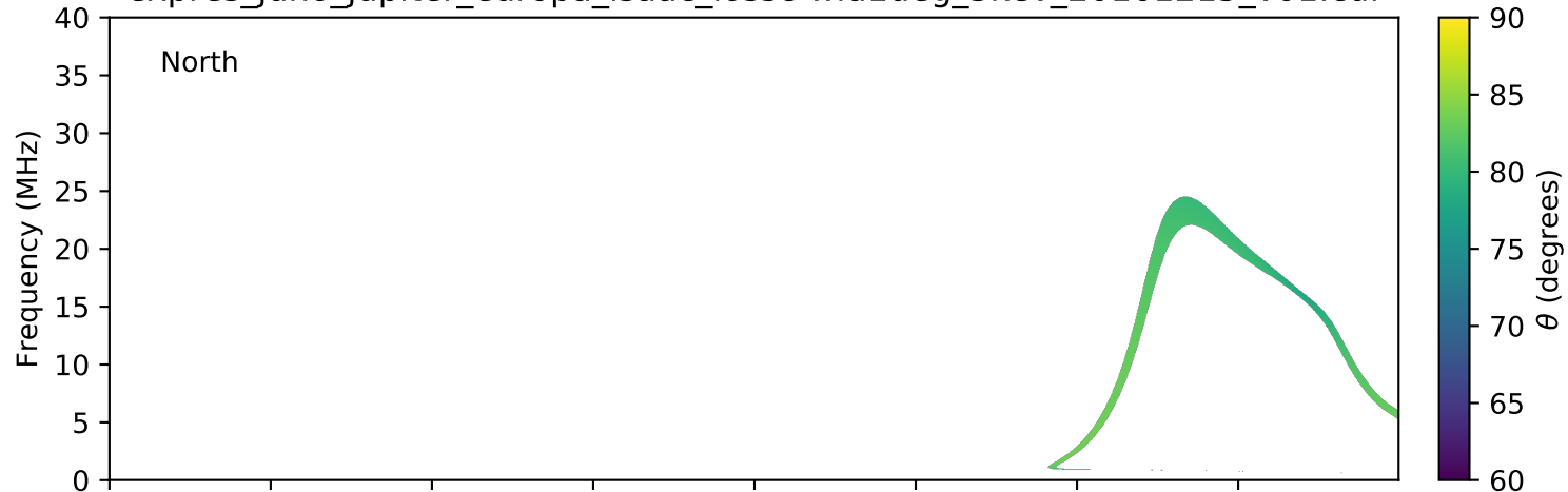
expres_juno_jupiter_europa_isaac_lossc-wid1deg_3kev_20161215_v01.cdf
