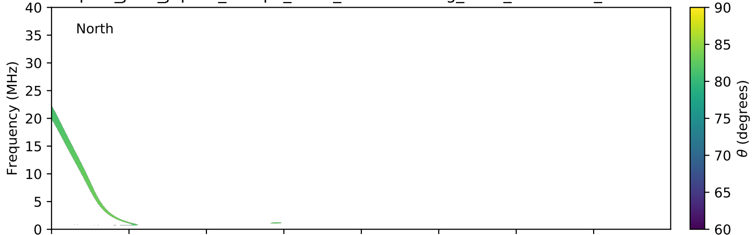
expres_juno_jupiter_europa_isaac_lossc-wid1deg_3kev_20161213_v01.cdf
