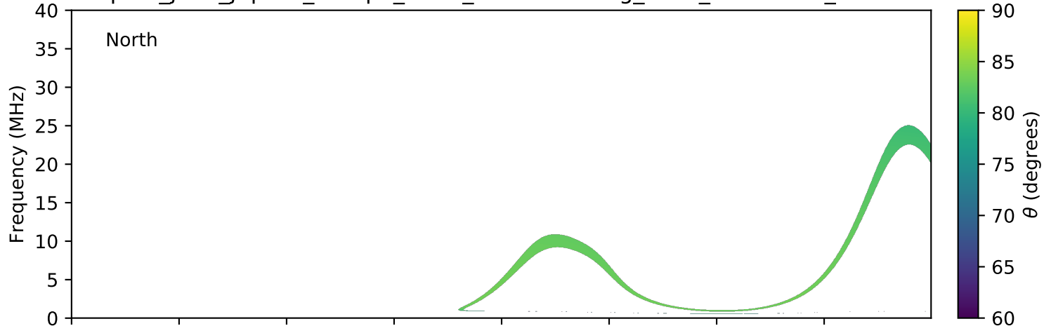
expres_juno_jupiter_europa_isaac_lossc-wid1deg_3kev_20161212_v01.cdf
