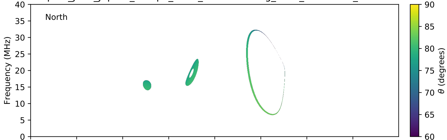
expres_juno_jupiter_europa_isaac_lossc-wid1deg_3kev_20161211_v01.cdf
