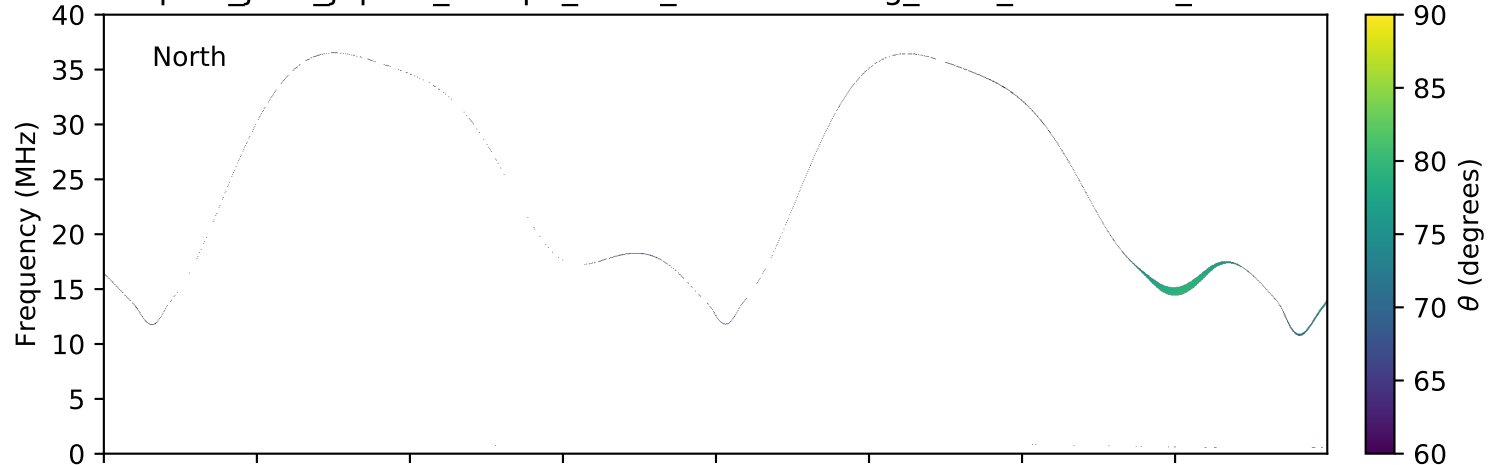
expres_juno_jupiter_europa_isaac_lossc-wid1deg_3kev_20161209_v01.cdf
