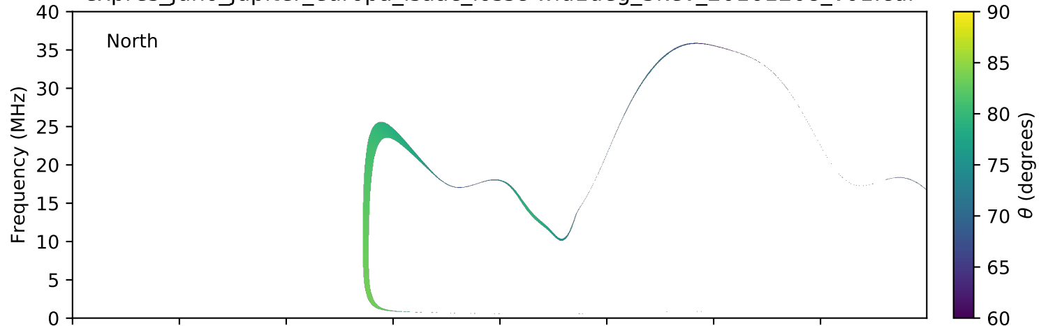
expres_juno_jupiter_europa_isaac_lossc-wid1deg_3kev_20161208_v01.cdf
