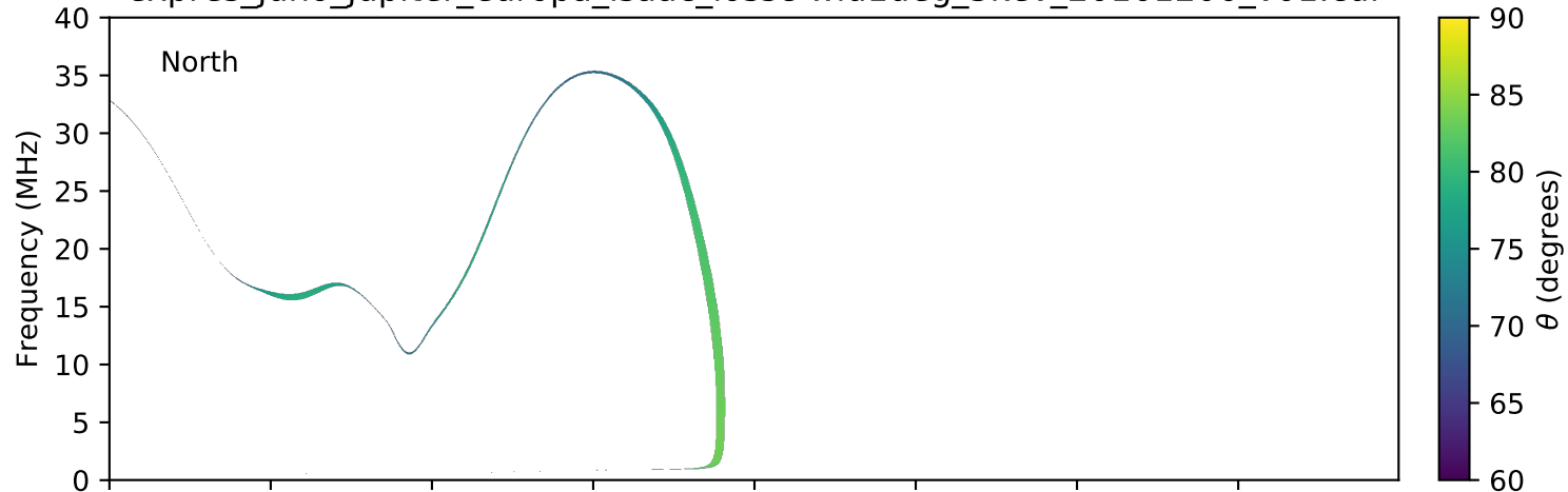
expres_juno_jupiter_europa_isaac_lossc-wid1deg_3kev_20161206_v01.cdf
