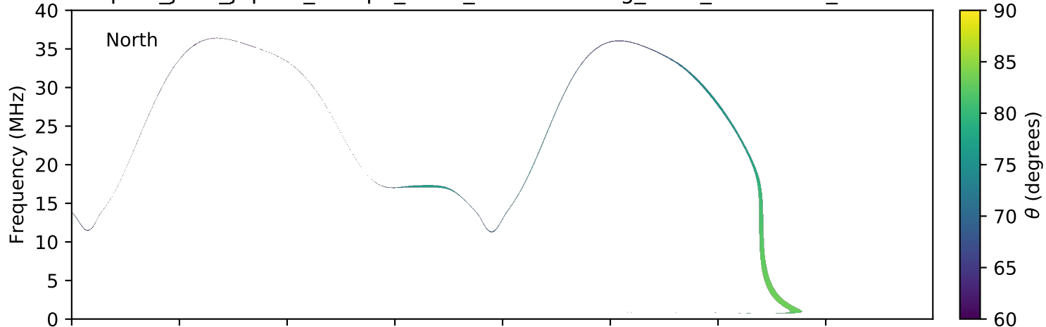
expres_juno_jupiter_europa_isaac_lossc-wid1deg_3kev_20161202_v01.cdf
