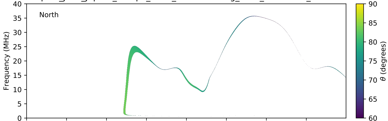
expres_juno_jupiter_europa_isaac_lossc-wid1deg_3kev_20161201_v01.cdf
