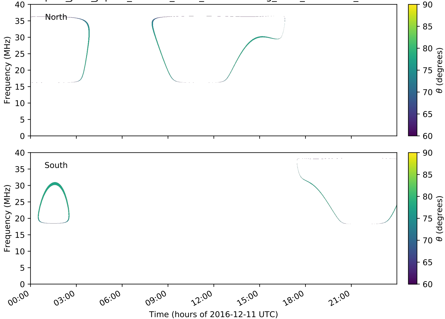
expres_juno_jupiter_340d-0r_isaac_lossc-wid1deg_9kev_20161211_v01.cdf
