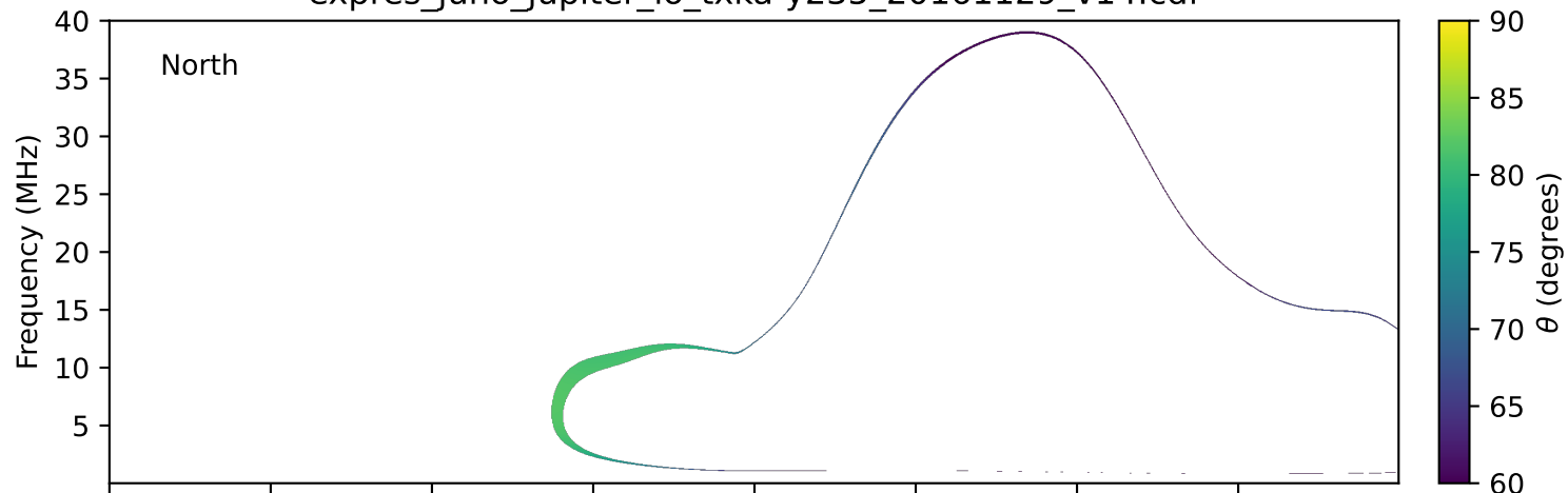
expres_juno_jupiter_io_txka-y235_20161129_v14.cdf
