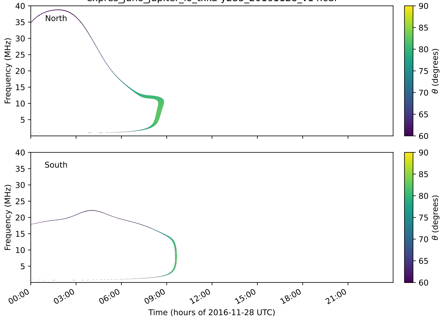
expres_juno_jupiter_io_txka-y235_20161128_v14.cdf
