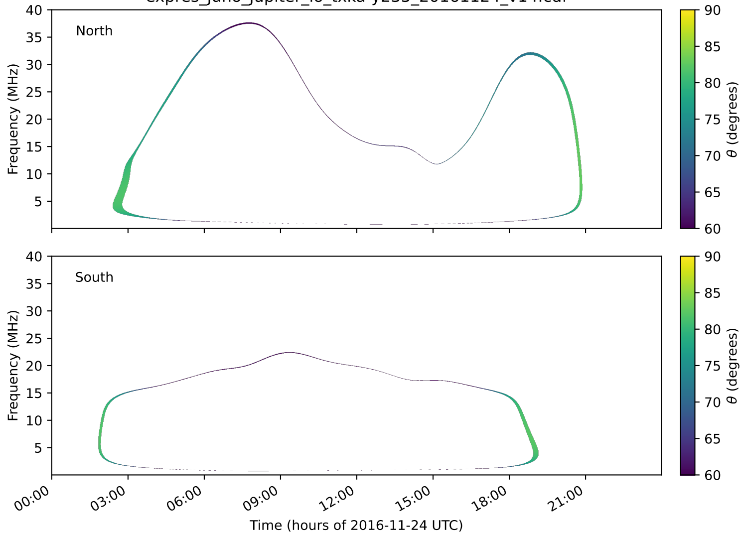
expres_juno_jupiter_io_txka-y235_20161124_v14.cdf
