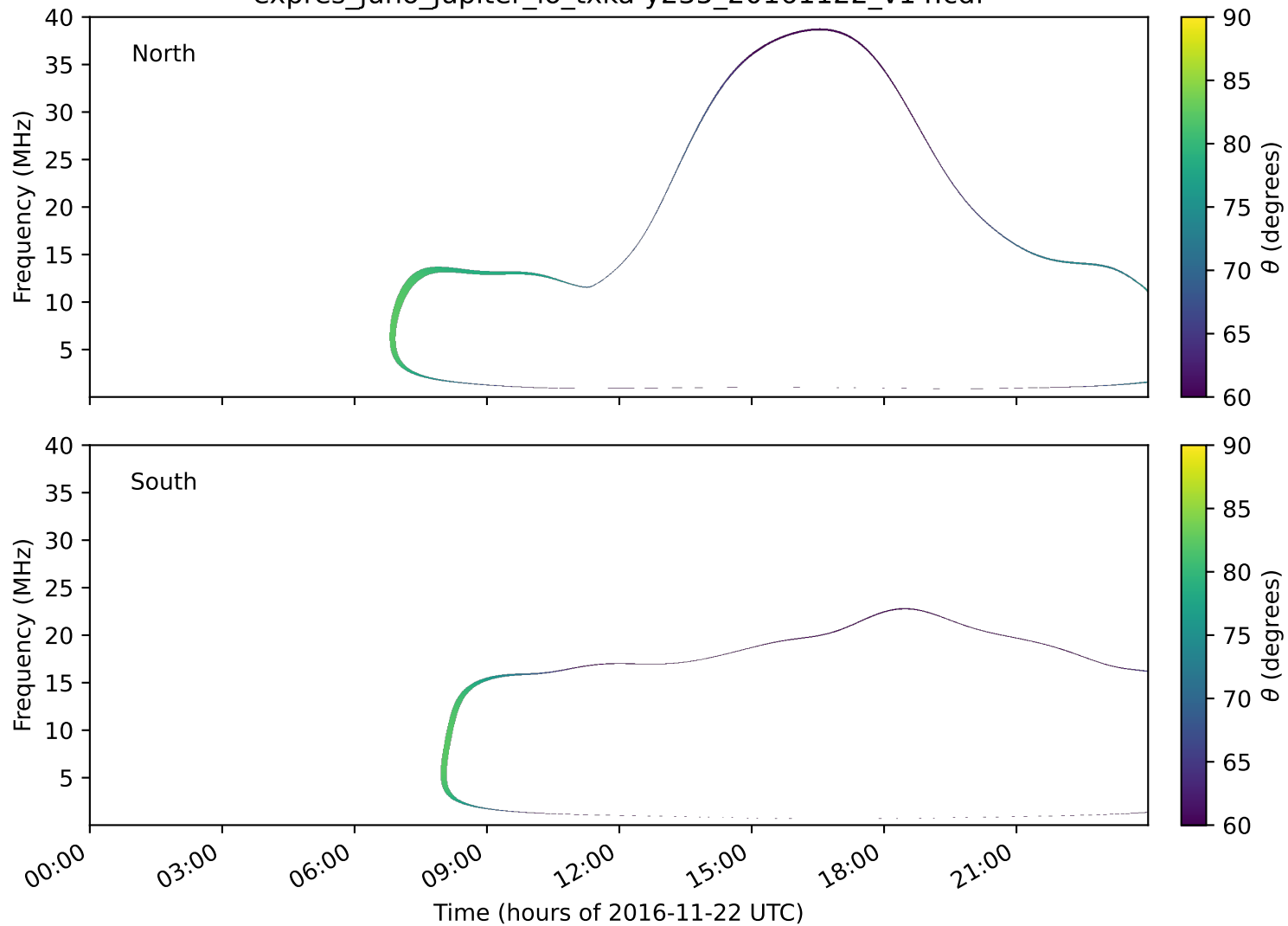
expres_juno_jupiter_io_txka-y235_20161122_v14.cdf
