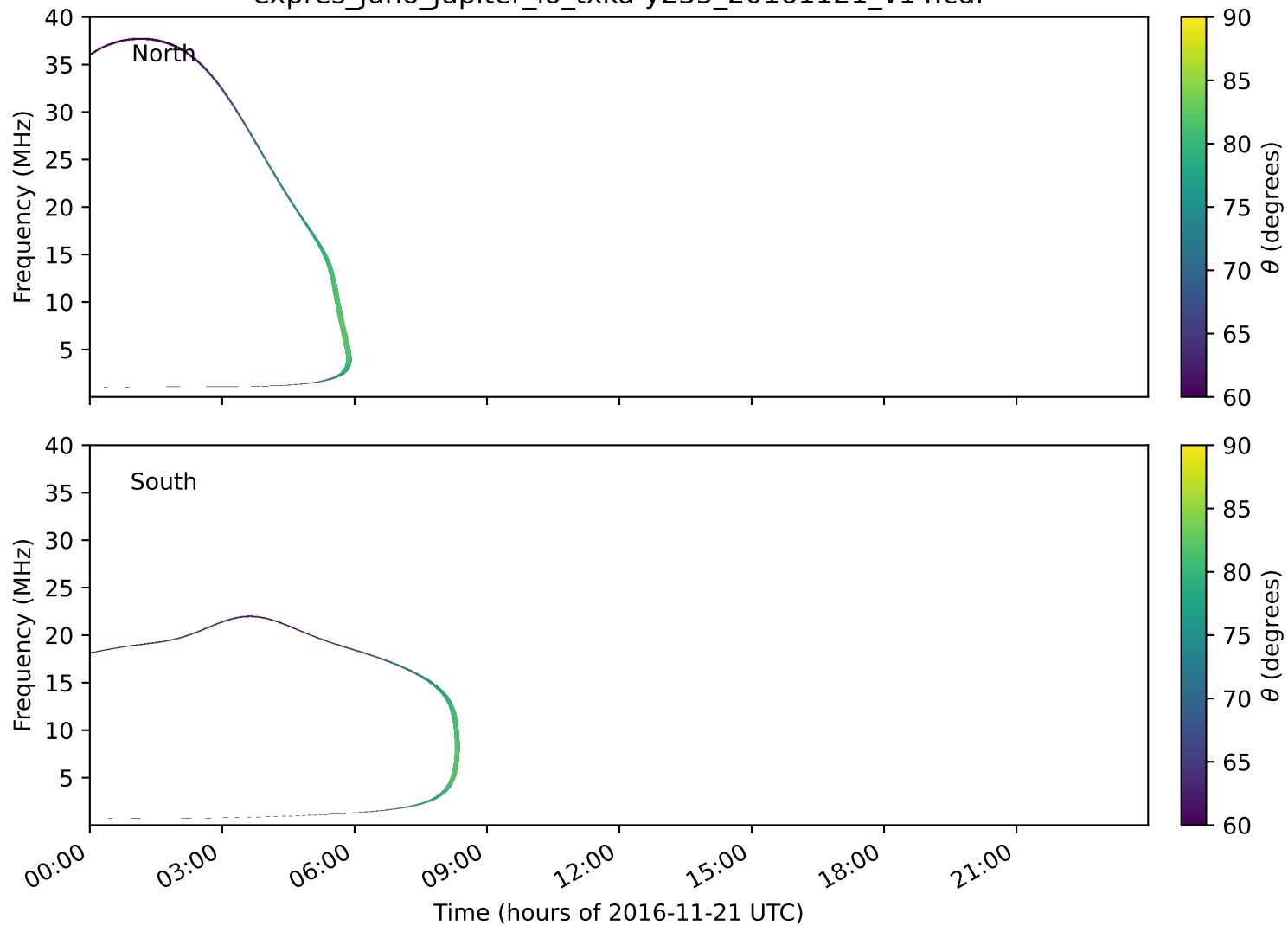
expres_juno_jupiter_io_txka-y235_20161121_v14.cdf
