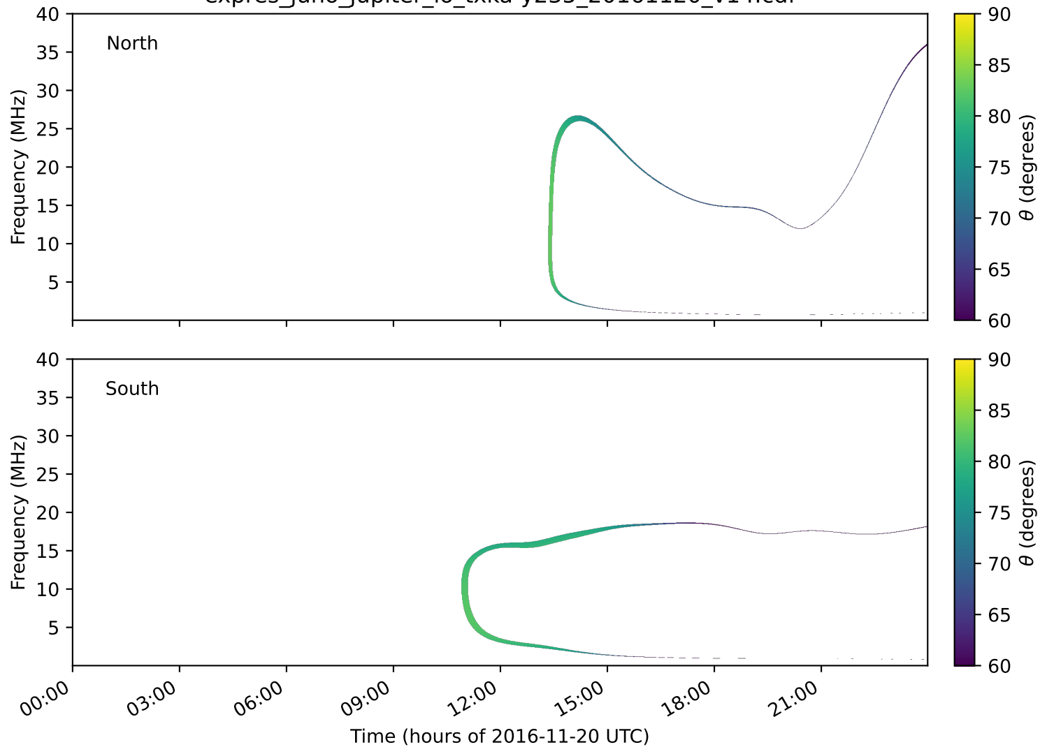
expres_juno_jupiter_io_txka-y235_20161120_v14.cdf
