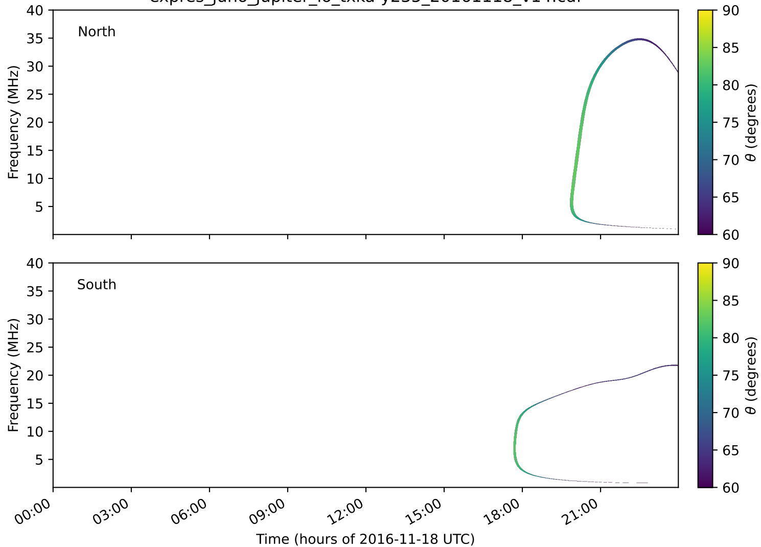
expres_juno_jupiter_io_txka-y235_20161118_v14.cdf
