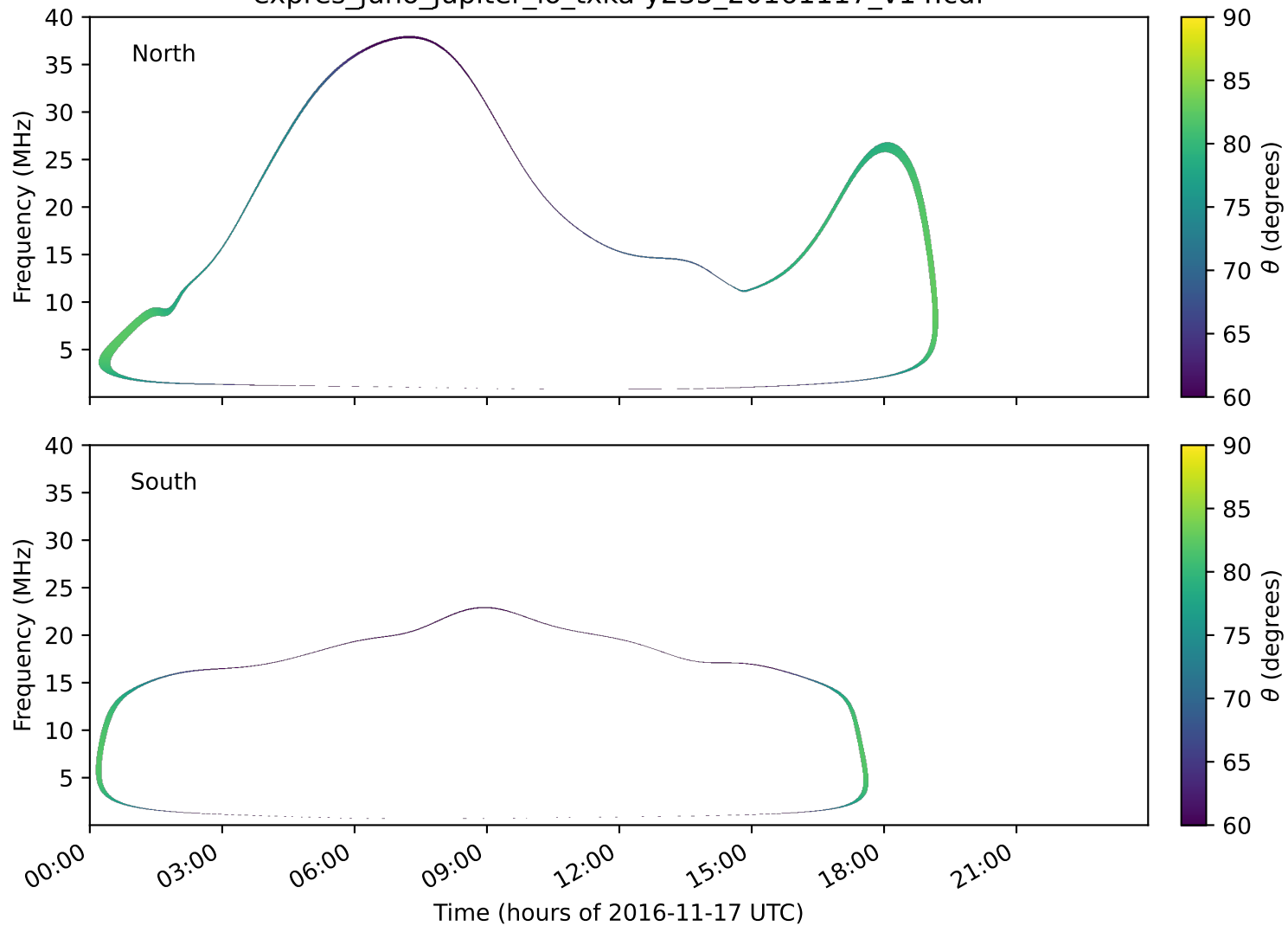
expres_juno_jupiter_io_txka-y235_20161117_v14.cdf
