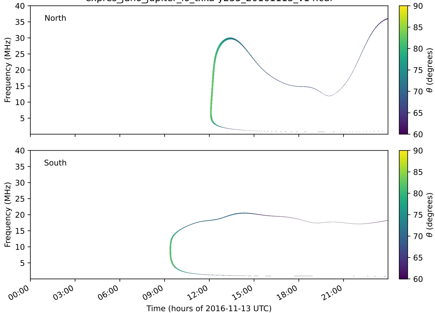
expres_juno_jupiter_io_txka-y235_20161113_v14.cdf
