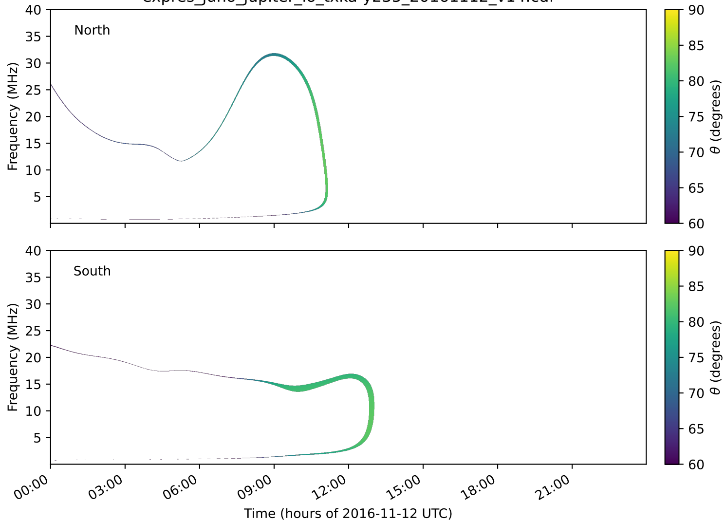
expres_juno_jupiter_io_txka-y235_20161112_v14.cdf
