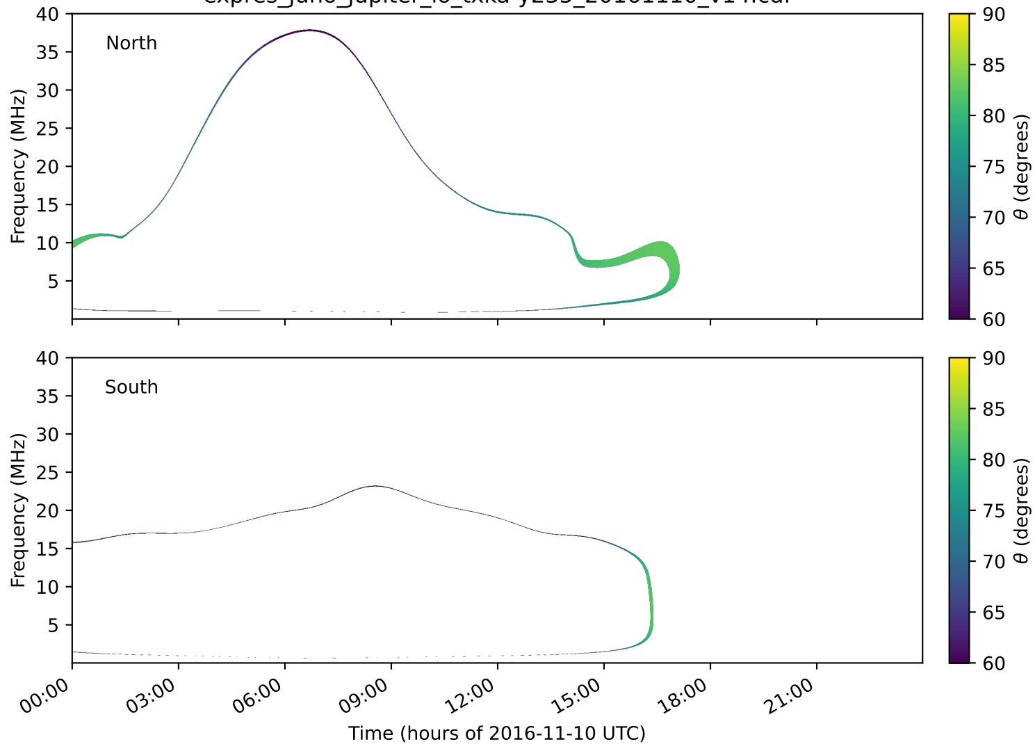
expres_juno_jupiter_io_txka-y235_20161110_v14.cdf
