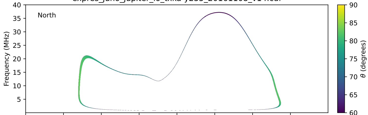
expres_juno_jupiter_io_txka-y235_20161108_v14.cdf
