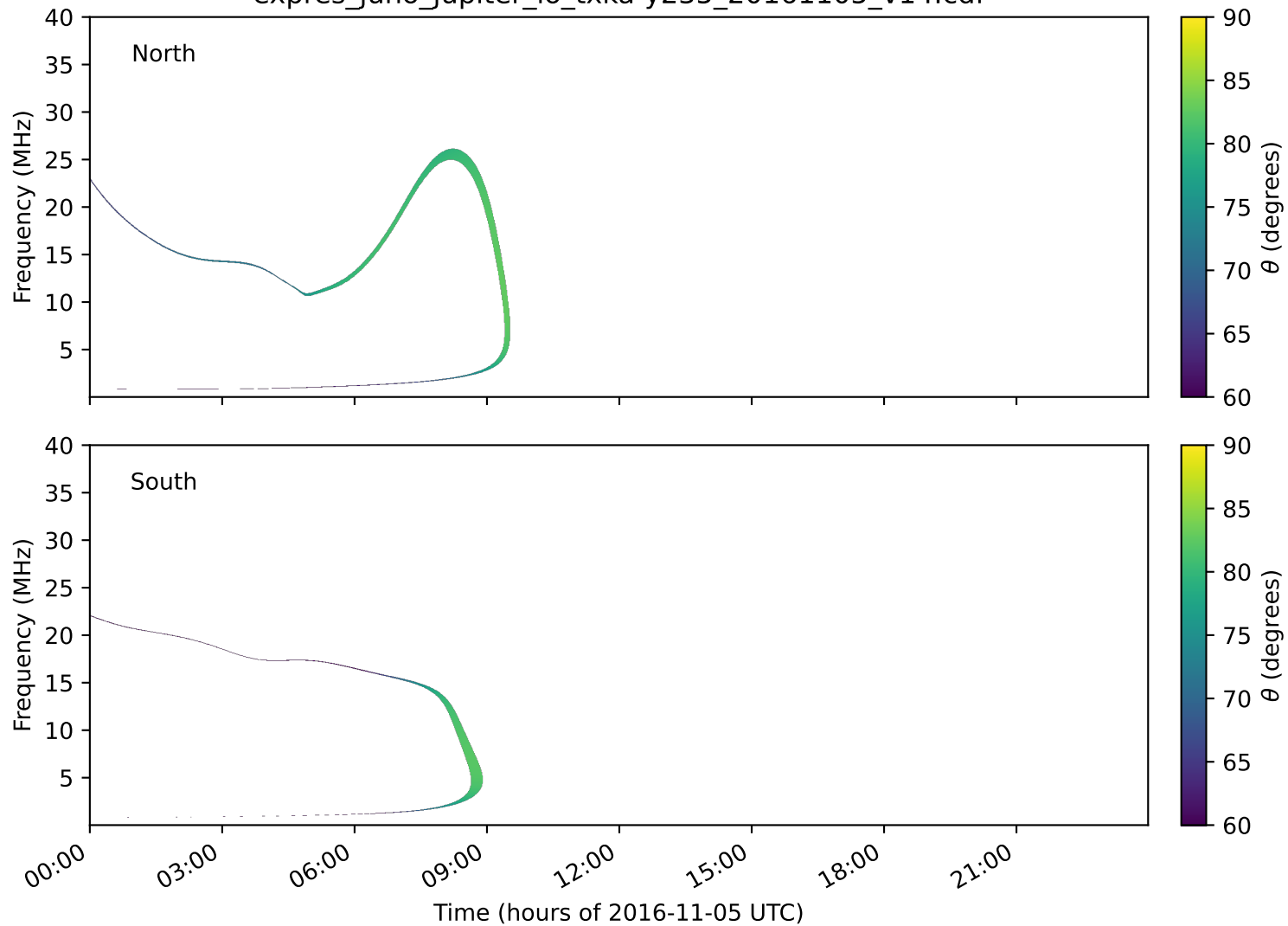
expres_juno_jupiter_io_txka-y235_20161105_v14.cdf
