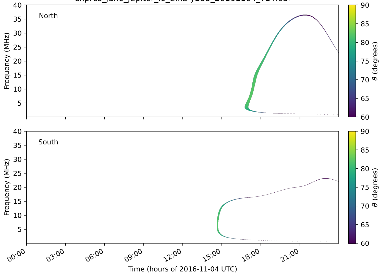
expres_juno_jupiter_io_txka-y235_20161104_v14.cdf
