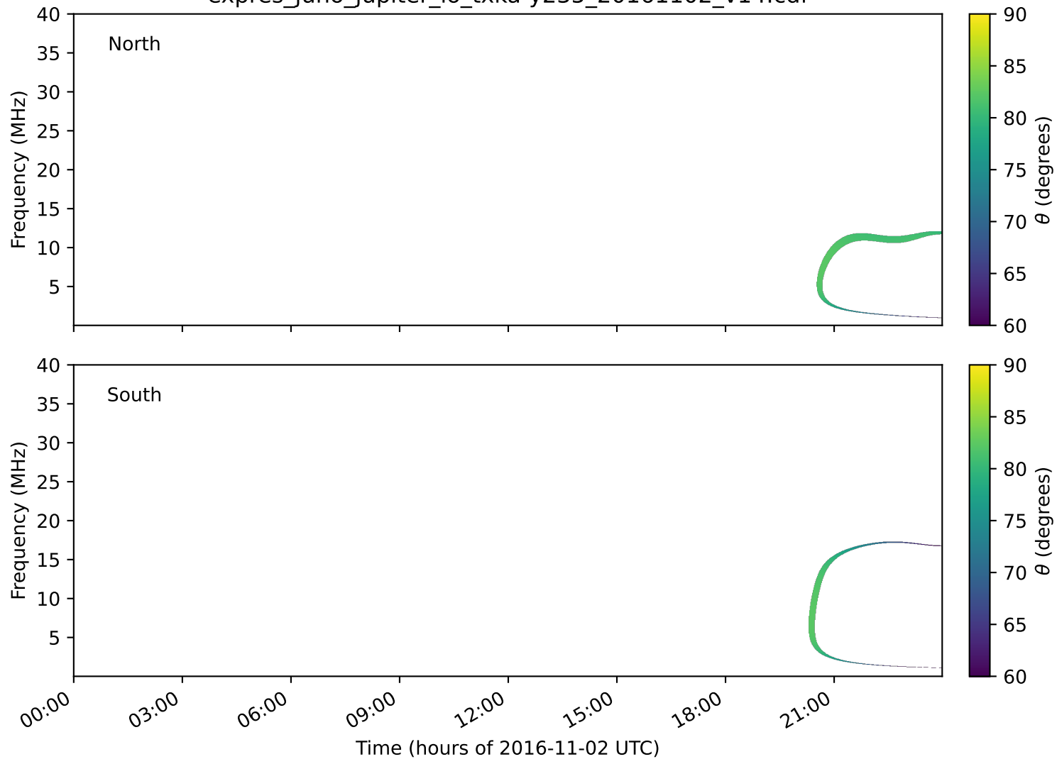
expres_juno_jupiter_io_txka-y235_20161102_v14.cdf
