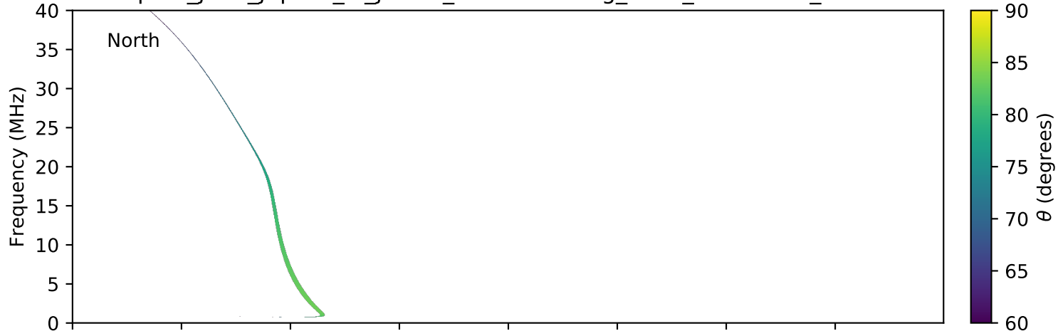
expres_juno_jupiter_io_jrm09_lossc-wid1deg_3kev_20161121_v01.cdf
