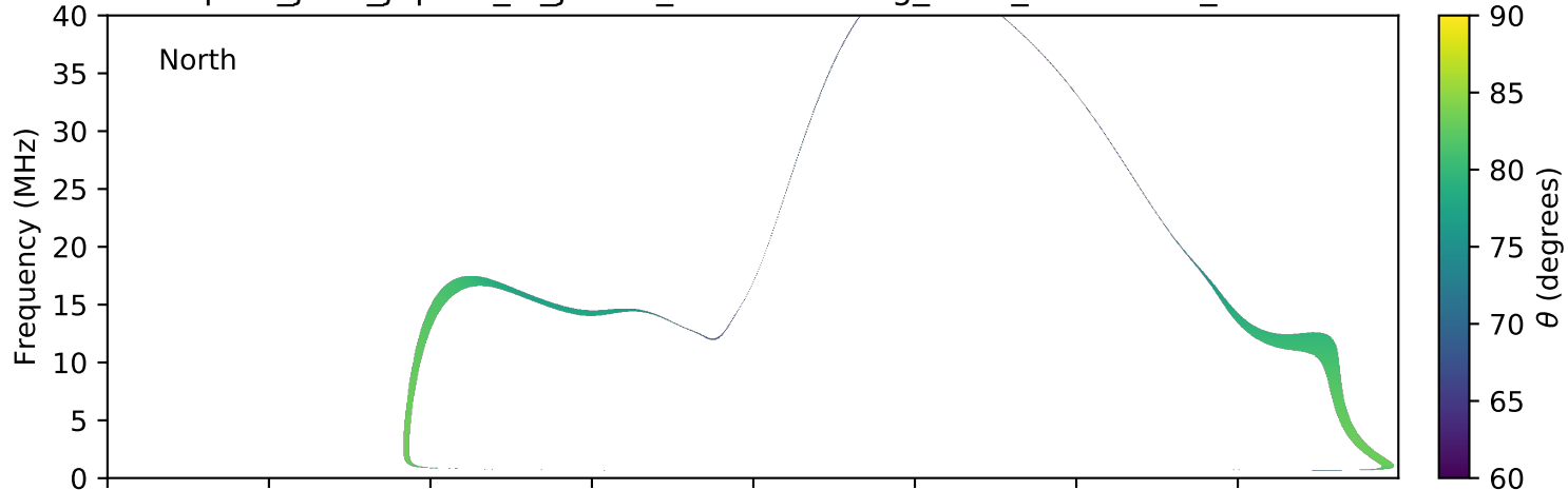
expres_juno_jupiter_io_jrm09_lossc-wid1deg_3kev_20161115_v01.cdf
