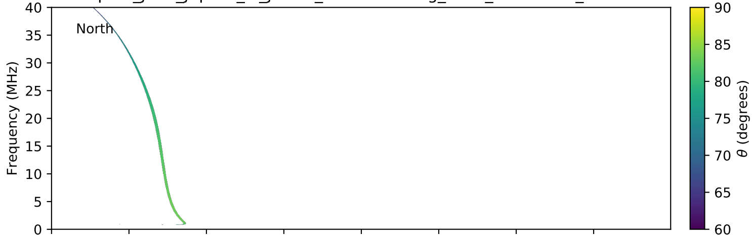
expres_juno_jupiter_io_jrm09_lossc-wid1deg_3kev_20161114_v01.cdf
