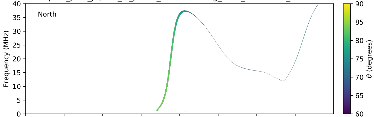
expres_juno_jupiter_io_jrm09_lossc-wid1deg_3kev_20161106_v01.cdf
