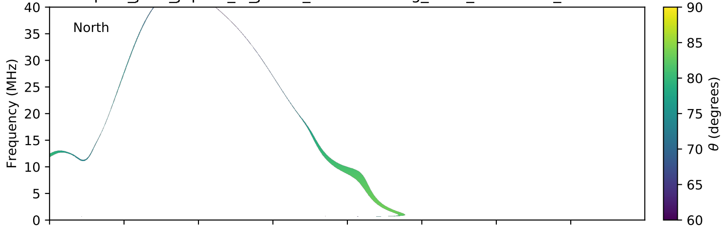
expres_juno_jupiter_io_jrm09_lossc-wid1deg_3kev_20161103_v01.cdf
