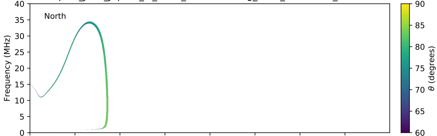
expres_juno_jupiter_io_isaac_lossc-wid1deg_3kev_20161130_v01.cdf
