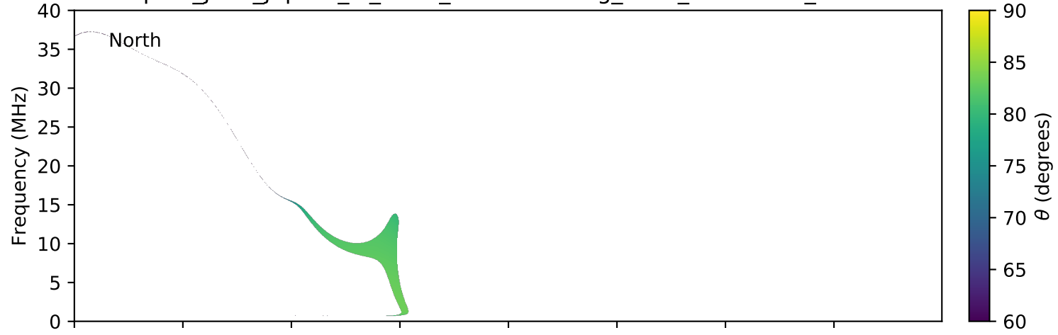
expres_juno_jupiter_io_isaac_lossc-wid1deg_3kev_20161128_v01.cdf
