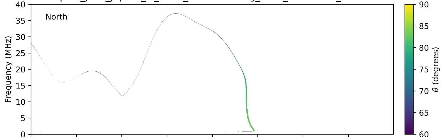
expres_juno_jupiter_io_isaac_lossc-wid1deg_3kev_20161126_v01.cdf
